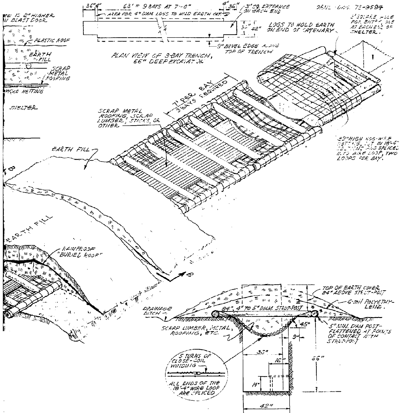
CROSS SECTION OF ELEVATION B-B
